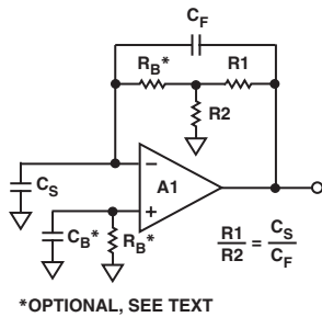
Figure 4. Charge Amplifier Circuit
