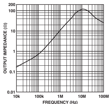
TPC 6. Output Impedance vs. Frequency (Closed-Loop Gain = -1)
